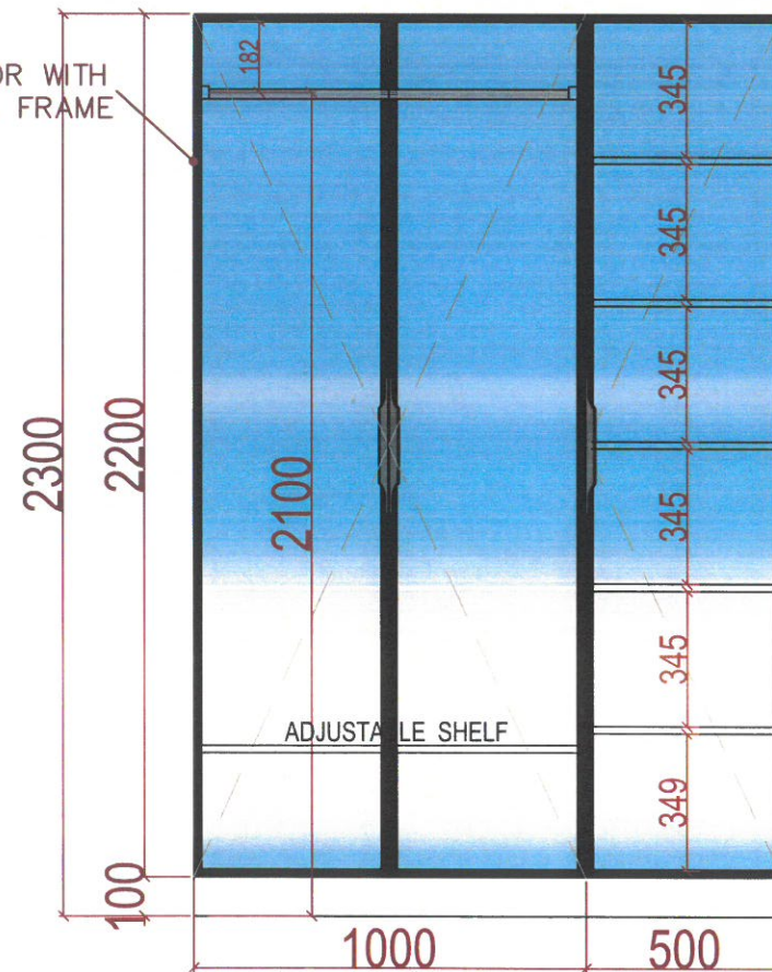
FRONT VIEW LOBBY-CLOSET
