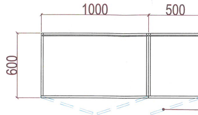
TOP VIEW LOBBY-CLOSET
