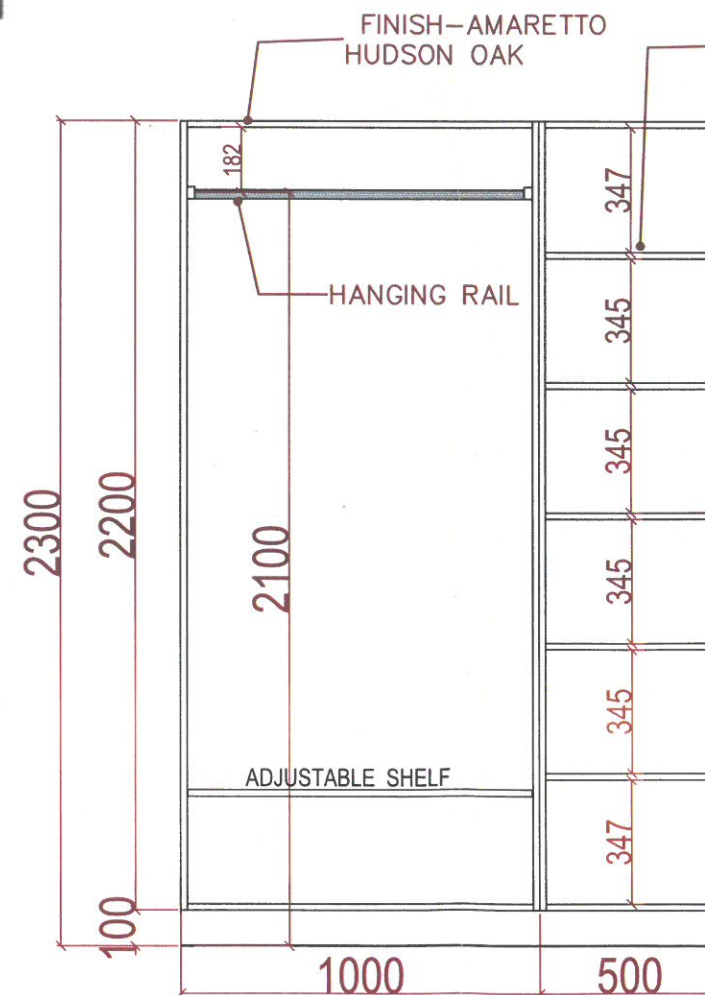
INNER VIEW LOBBY-CLOSET
